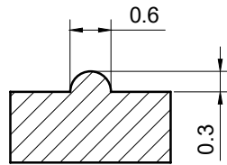
DETAIL-I (IDENTIFICATION MARK)
