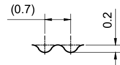
DETAIL - F SCALE 10:1
