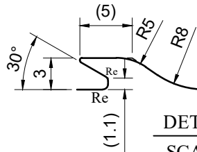
DETAIL-I (IDENTIFICATION MARK)
